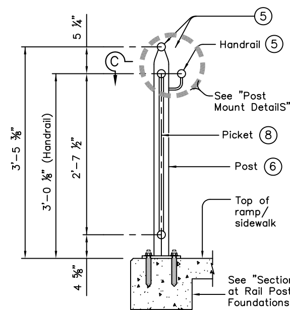
SECTION B - B (Showing Handrail OPTION "2")
