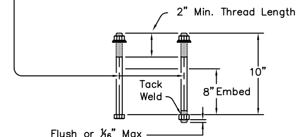
CAST-IN-PLACE ANCHOR BOLT OPTIONS
