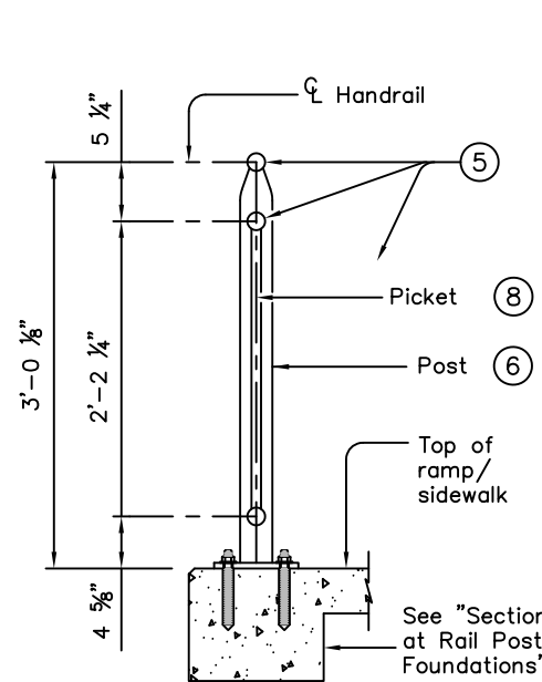
SECTION A - A (Showing Handrail OPTION "1")
