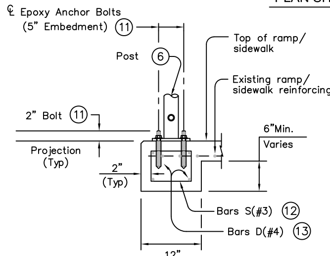
WITHOUT CURB
