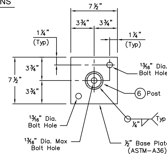
TYPICAL POST BASE PLATE DETAIL
