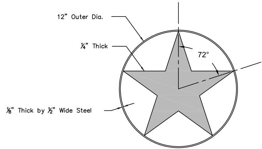
STAR DETAIL
