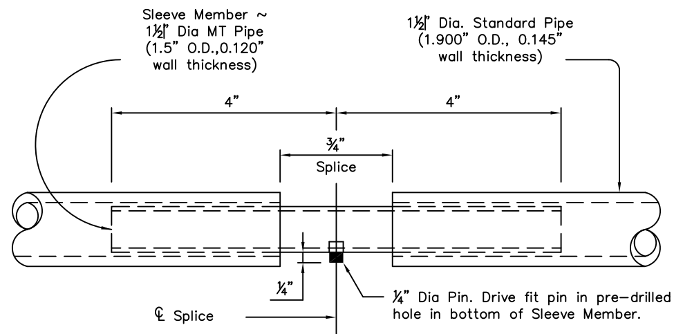
AT SPLICE JOINTS
