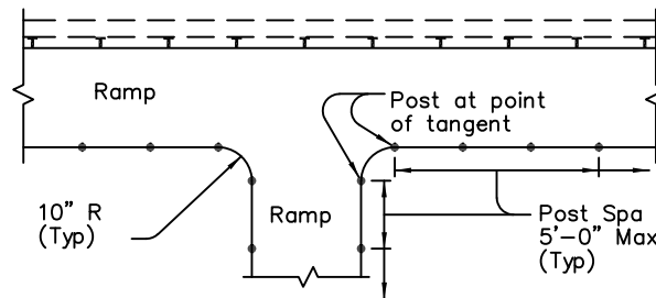
RAMP INTERSECTION
