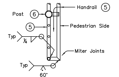
SECTION C - C (Showing Handrail Termination)
