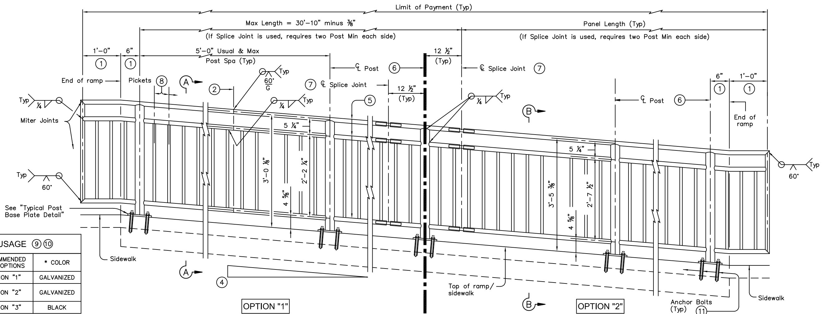
ELEVATION VIEW
