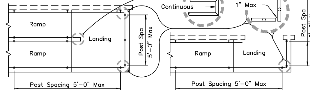
MULTI-LEVEL RAMP
